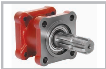
Code: 500 050 01 PRODUCTS : POWER TAKE OFF PUMP EXTENSION SHORT TRACTOR CASTING
