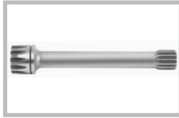
Code: 151 213 045 PRODUCTS : 15 S 151 CARDAN SHAFT 213 MM.
