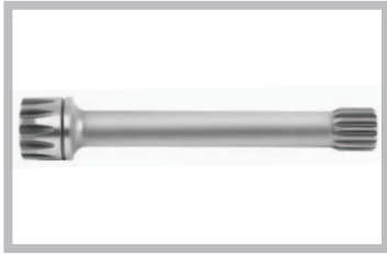
Code: 151 200 045 PRODUCTS : 15 S 151 CARDAN SHAFT 200 MM.
